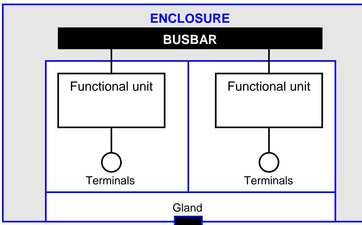
Figure 13.6 graphical description of Form 4a : Terminals in same compartment as associated functional unit (common glanding):
